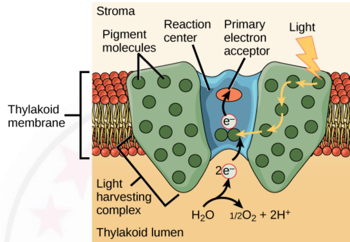
(a) Photosystem II (P680)
