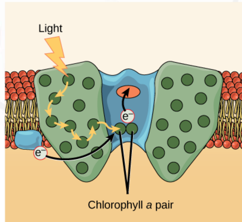
(b) Photosystem I (P700)
